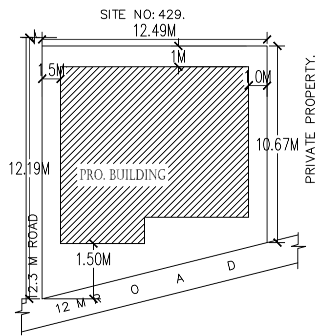
SITE PLAN
